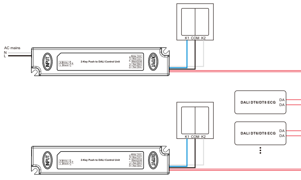
Figure 2: Wiring scheme to control up to 50 DALI ECGs (2 control units powered by AC mains, 3 control units powered by AC mains for 75 DALI ECGs, 4 control units powered by AC mains for 100 DALI ECGs)
